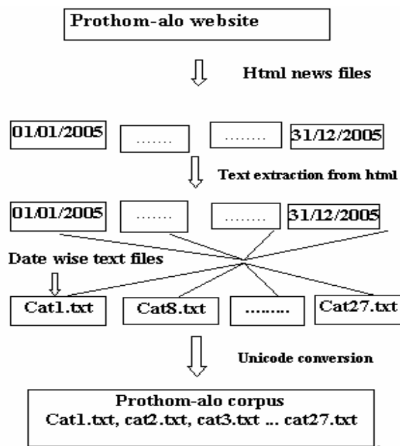
Figure 1: Compilation steps of Prothom-Alo corpus
